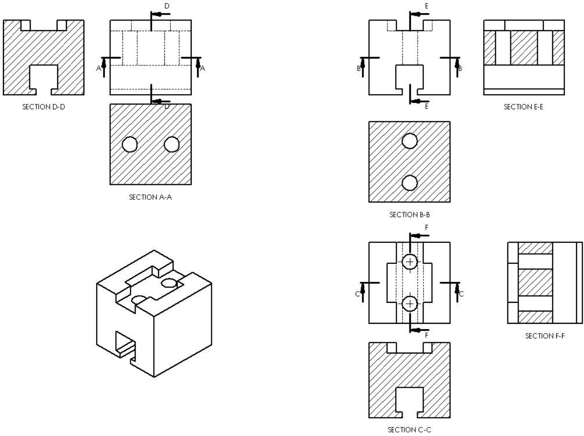
SEC C-C
